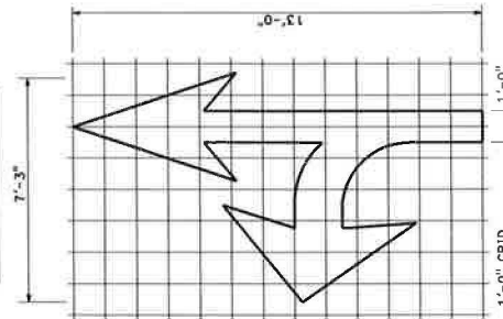
TYPE VIII ARROW A=36 f+2
